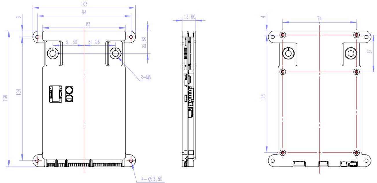
JK-BD6AxxS-6PT/8PT外形尺寸
