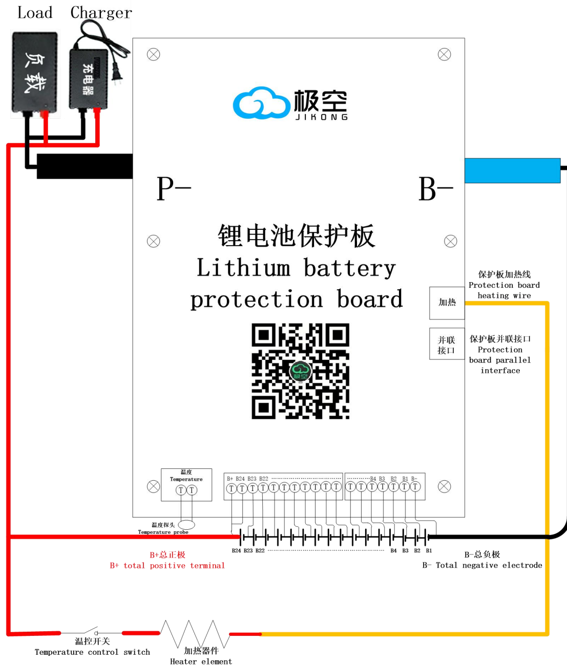
JK-BD4AxxS-6P/8P-24S接线图
