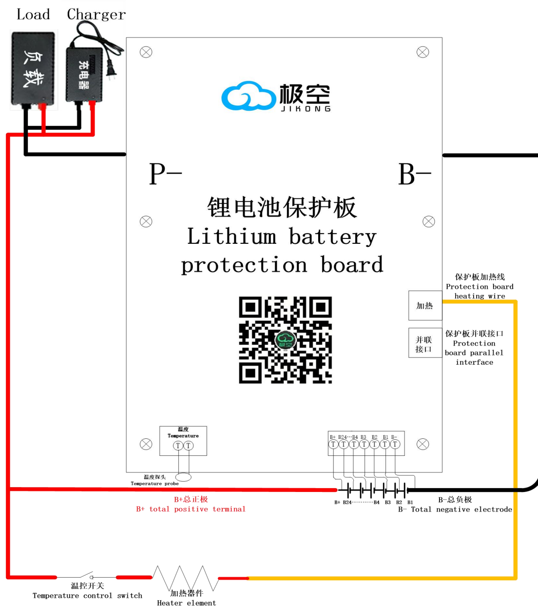
JK-BD4AxxS-10P-24S接线图
