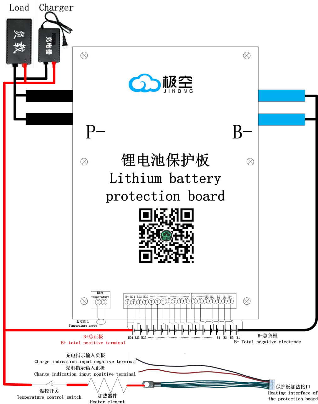
JK-BD4AxxS-10P-24S接线图
