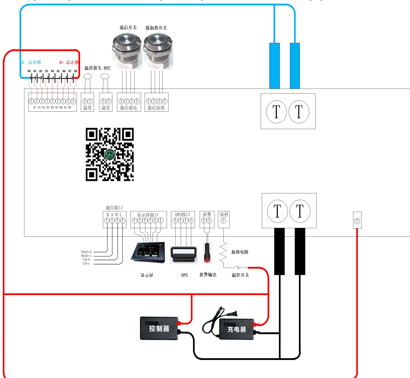
JK-QB2A8S-20P 接线图
