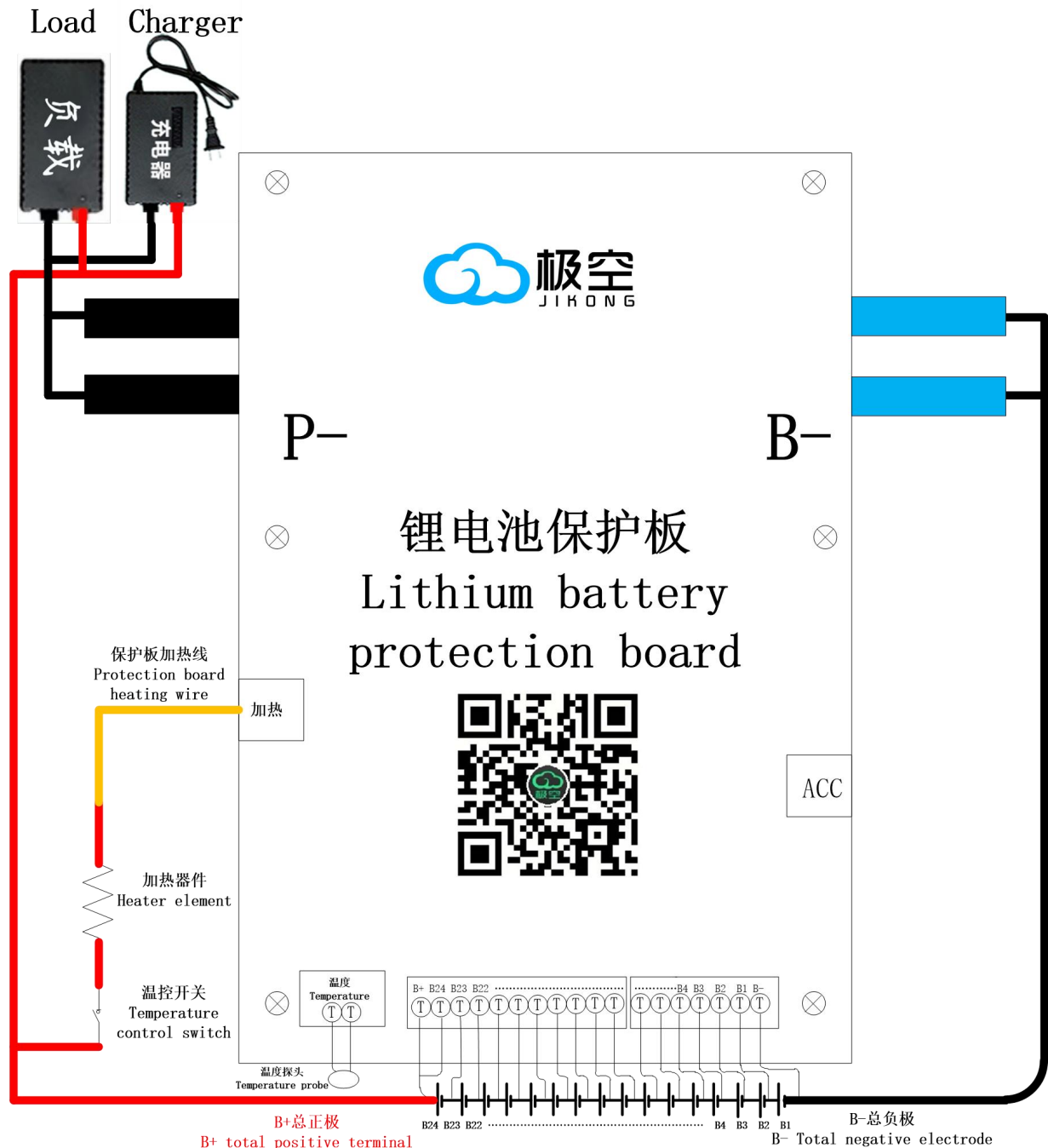
JK-BD4AxxS-10P-24S接线图
