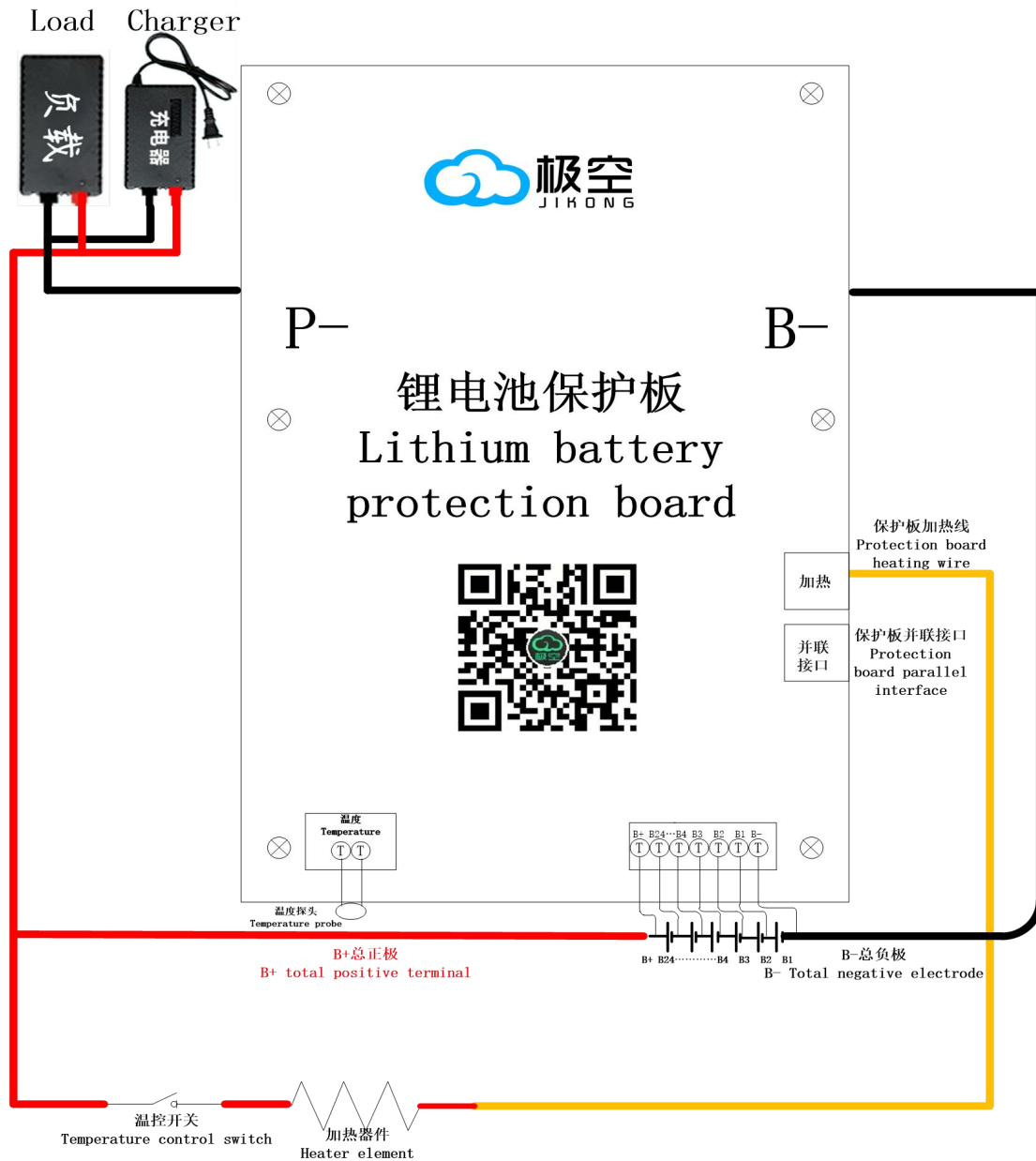
JK-BD4AxxS-10P-24S接线图 JK-BD4AxxS-10P-24S wiring diagram
